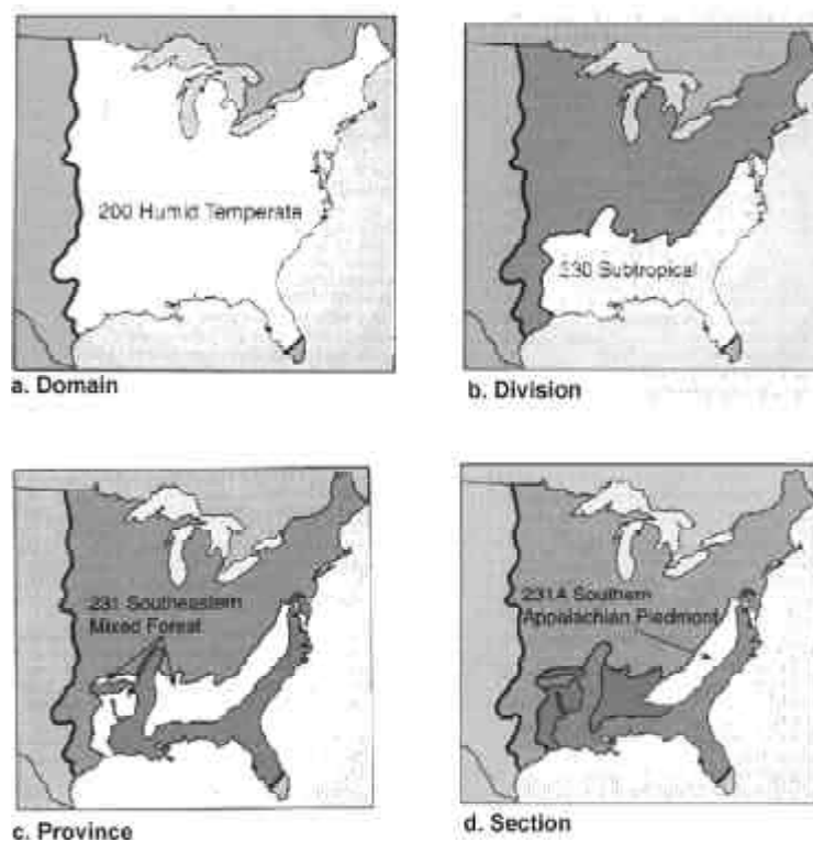
FIGURE 3: EXAMPLES OF FIRST FOUR HIERARCHICAL LEVELS OF ECOLOGICAL UNITS: DOMAIN, DIVISION, PROVINCE, AND SECTION, FROM US EPA ENVIRONMENTAL ATLAS.
